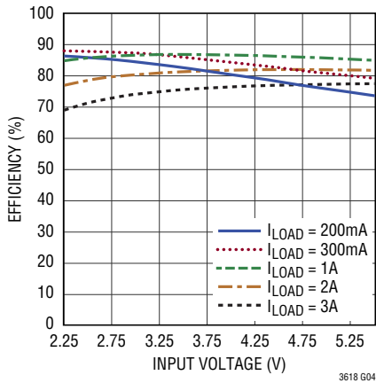
Efficiency vs Input Voltage V_{\text{TT}} = 0.9\text{V}
