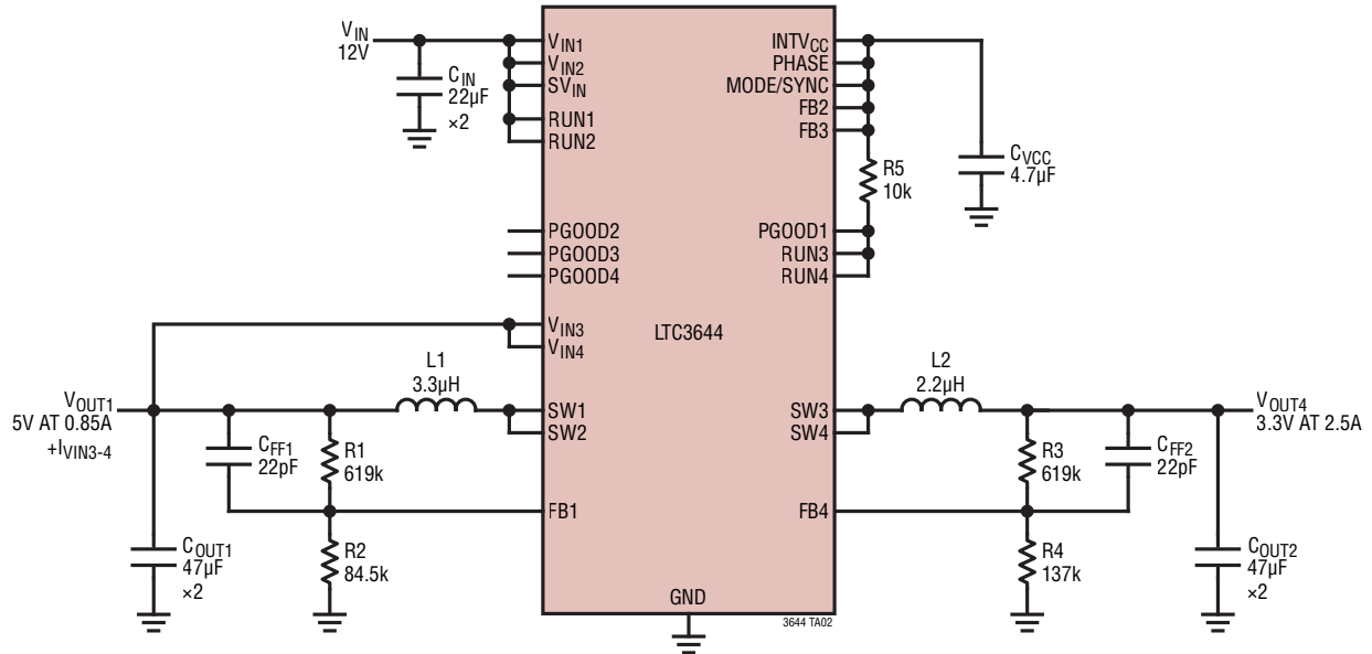
0.85A/2.5A Series Output 1MHz Step-Down Regulator
