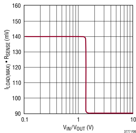
Figure 6. Load Current vs V_{\text{IN}}/V_{\text{OUT}}
