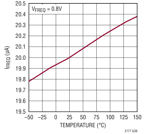
Frequency Setting Current vs Temperature
