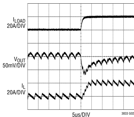
LOAD STEP = 0A TO 20A V_{IN} = 12V , V_{OUT} = 1.5V FIGURE 10 CIRCUIT
