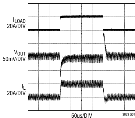
LOAD TRANSIENT = 0A TO 20A V_{IN} = 12V , V_{OUT} = 1.5V FIGURE 10 CIRCUIT
