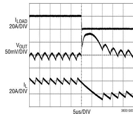
LOAD RELEASE = 20A TO 0A V_{IN} = 12V , V_{OUT} = 1.5V FIGURE 10 CIRCUIT
