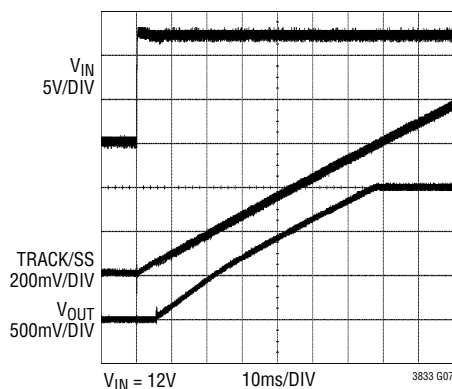
V_{IN} = 12V V_{OUT} = 1.5V FIGURE 10 CIRCUIT
