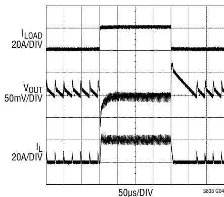
LOAD TRANSIENT = 500mA TO 20A V_{IN} = 12V , V_{OUT} = 1.5V FIGURE 10 CIRCUIT
