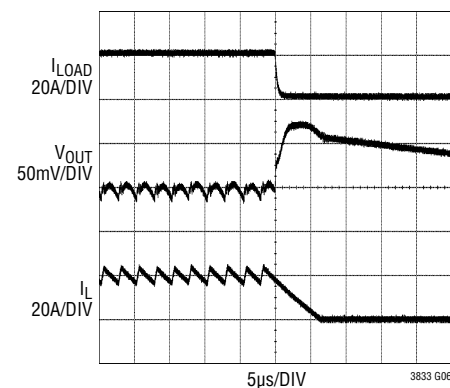
LOAD RELEASE = 20A TO 500mA V_{IN} = 12V , V_{OUT} = 1.5V FIGURE 10 CIRCUIT
