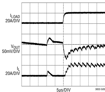
LOAD STEP = 500mA TO 20A V_{IN} = 12V , V_{OUT} = 1.5V FIGURE 10 CIRCUIT
