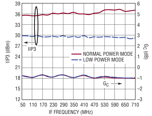
Conversion Gain and IIP3 vs IF Frequency (Low Side LO)
