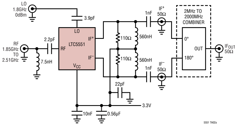
Wideband 100Ω Differential IF Output Matching
