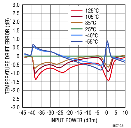
Linearity Error Temperature Variation from 25°C at 1GHz
