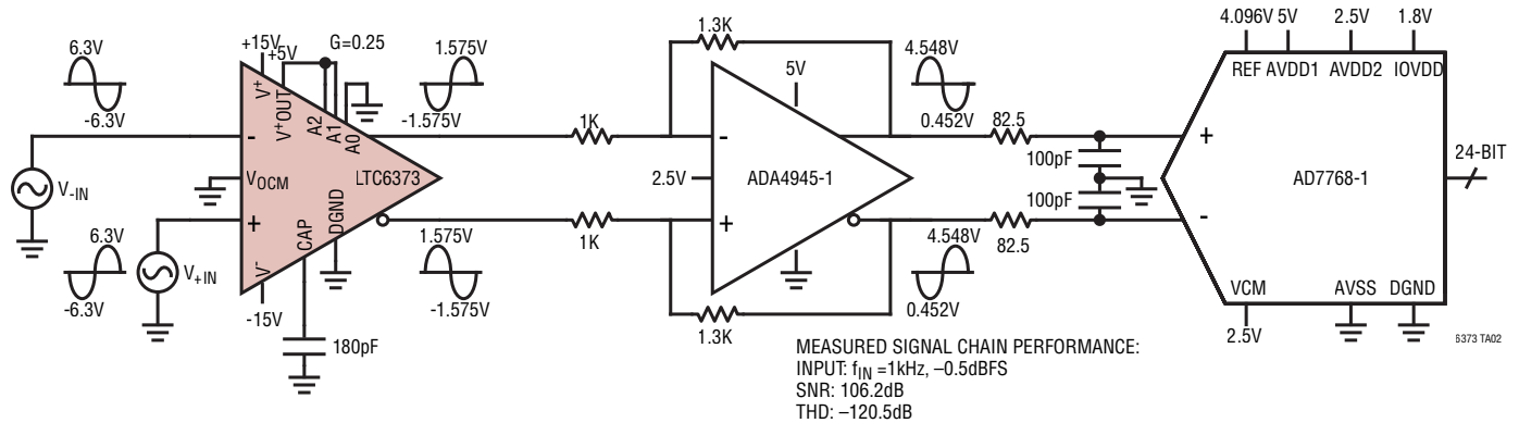
LTC6373 Driving the AD7768-1 \Sigma - \Delta ADC through a Fully Differential ADC Driver (ADA4945-1)
