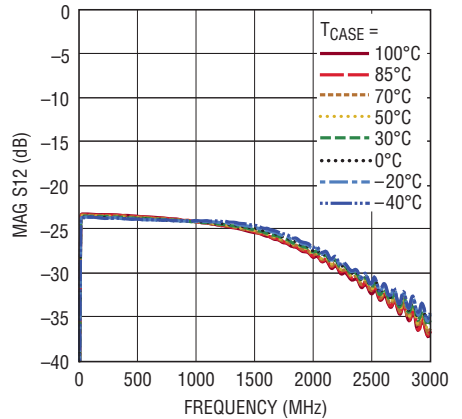
S12 vs Frequency Over Temperature
