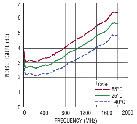
NF vs Frequency Over Case Temperature
