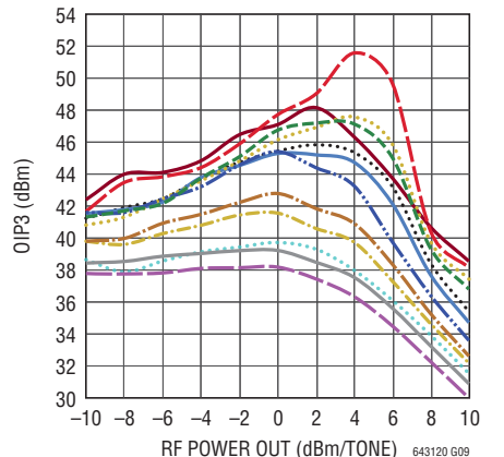
OIP3 vs Power Out Over Frequency
