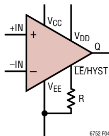
Figure 4. Adjusting Hysteresis Using an External Resistor at the \overline{\text{LE}}/\text{HYST} Pin
