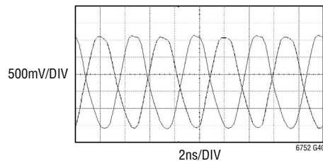
Output Toggle Waveforms Q and Q, LTC6752-3
