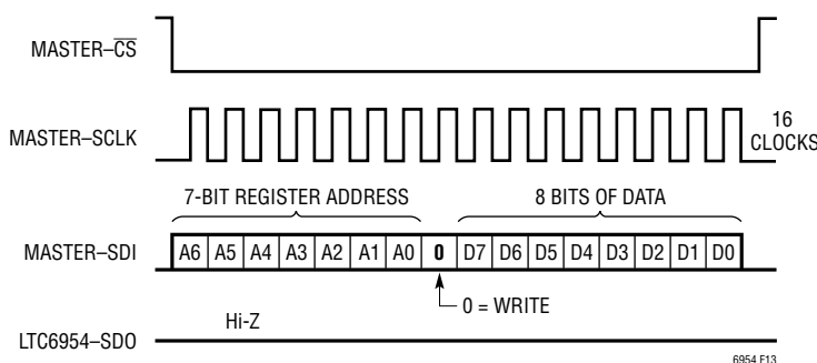
Figure 13. Serial Port Write Sequence
