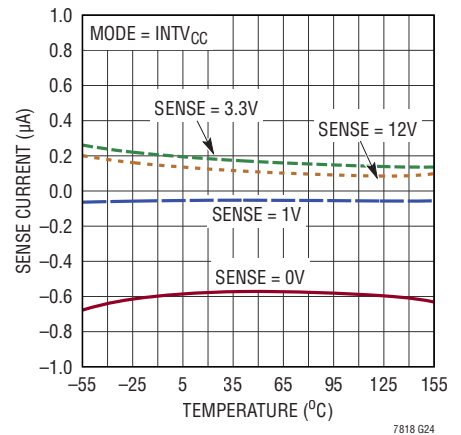
SENSE1,2 + and SENSE3 - Input Current vs Temperature
