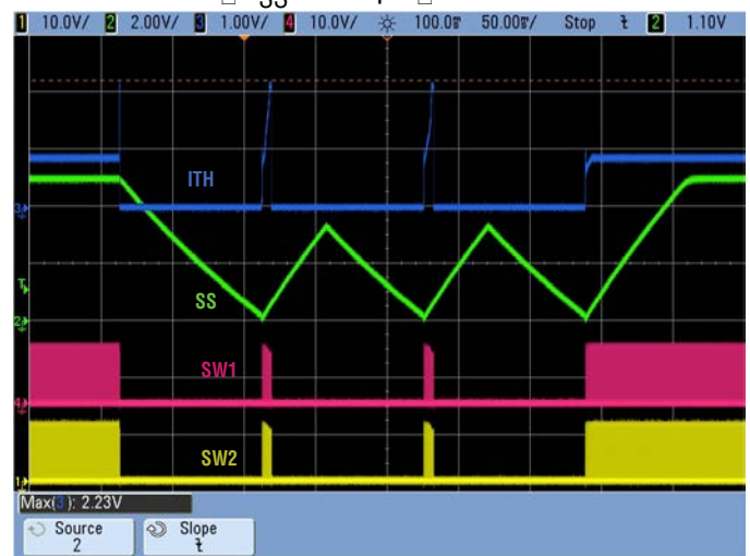
Figure 5. Hiccup Mode Overcurrent Protection and Recovery
