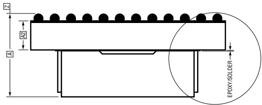
PACKAGE SIDE VIEW
