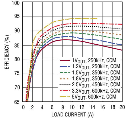
Efficiency vs Load Current with 12V IN (Limit 5V Output to 15A)
