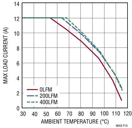
Figure 14. 5V IN to 1.0V OUT Derating Curve, 4-Channel Paralleled, No Heat Sink
