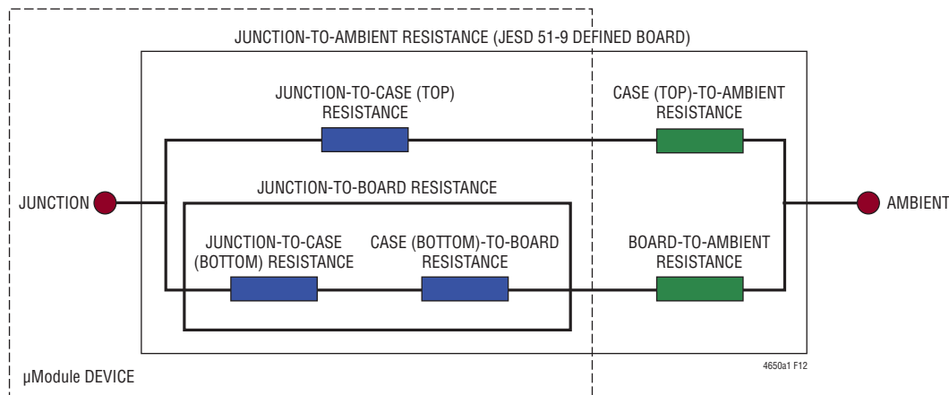
Figure 12. Graphical Representation of JEDEC Thermal Coefficients
