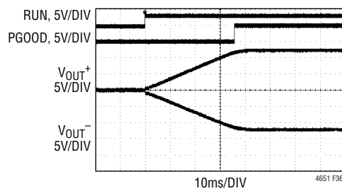
Figure 36. Concurrent ±12V Supply, Output Voltage Start-Up Waveforms. Figure 37 Circuit
