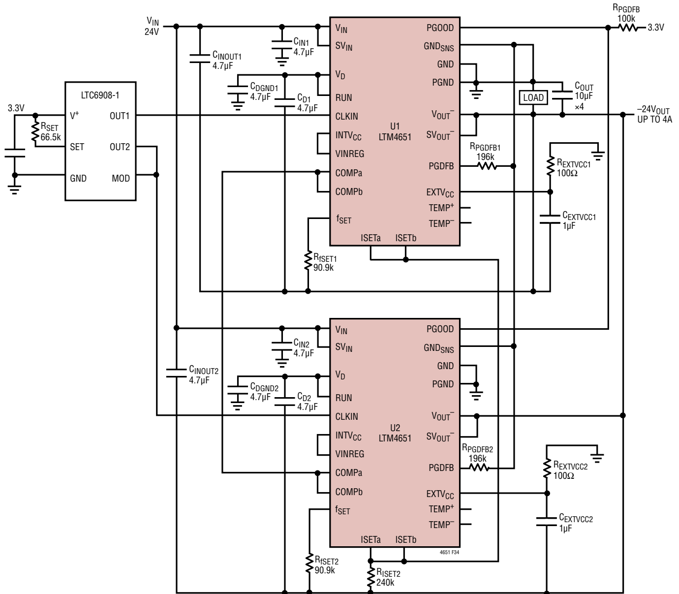
Figure 34. -24V Output at Up to 4A from 24V Input, 2-Phase Interleaved, Parallel Application at f_{SW} = 1.5MHz
