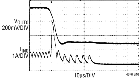
FIGURE 44 CIRCUIT AT 12\text{V}_{\text{IN}} , 77\text{m}\Omega LOAD ON V_{\text{OUTO}} PRIOR TO APPLICATION OF SHORT CIRCUIT
