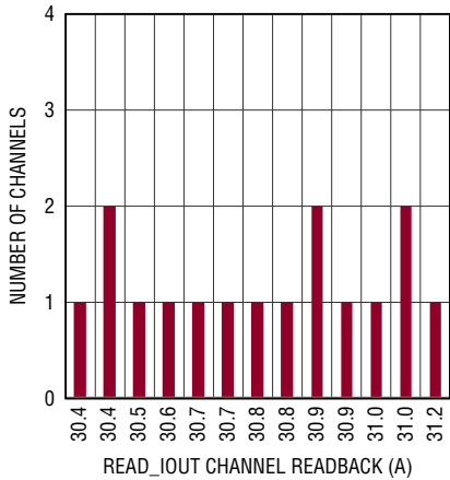
READ_IOUT of 16 LTM4680 Channels 12\text{V}_{\text{IN}} , 1\text{V}_{\text{OUT}} , T_J = -40^\circ\text{C} , I_{\text{OUT}\pi} = 30\text{A} , System Having Reached Thermally Steady-State Condition, No Airflow
