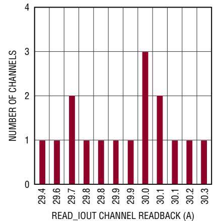
READ_IOUT of 16 LTM4680 Channels 12\text{V}_{\text{IN}} , 1\text{V}_{\text{OUT}} , T_J = 125^\circ\text{C} , I_{\text{OUT}\pi} = 30\text{A} , System Having Reached Thermally Steady-State Condition, No Airflow
