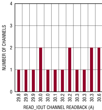
READ_IOUT of 16 LTM4680 Channels 12\text{V}_{\text{IN}} , 1\text{V}_{\text{OUT}} , T_J = 25^\circ\text{C} , I_{\text{OUT}\pi} = 30\text{A} , System Having Reached Thermally Steady-State Condition, No Airflow
