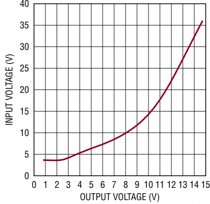
Minimum Input Running Voltage vs V_{OUT} , I_{OUT} = 3A
