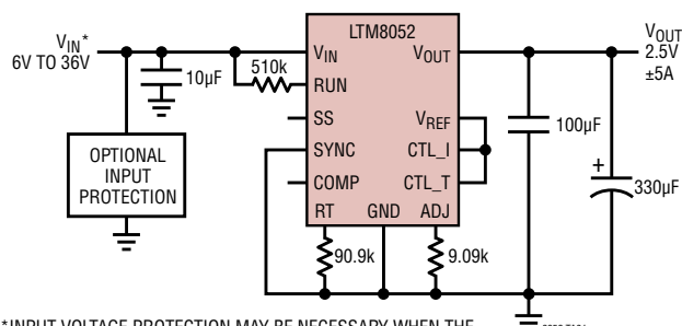
±5A, 2.5V (2-Quadrant) μModule Voltage Regulator
