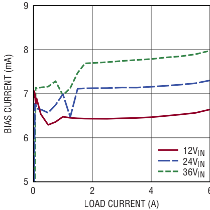
LTM8053 BIAS Current vs Load Current, V_{OUT} = 5V , BIAS = 5V
