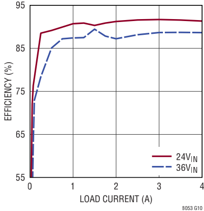
LTM8053 Efficiency vs Load Current, V_{OUT} = -5\text{V} , BIAS Tied to LTM8053 GND
