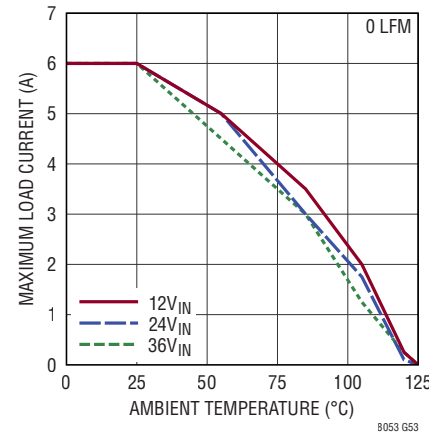
LTM8053 Derating, V_{OUT} = 2.5\text{V} , BIAS = 5V, DC1934A Demo Board
