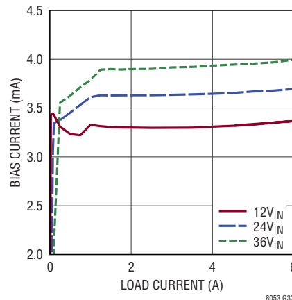
LTM8053 BIAS Current vs Load Current V_{OUT} = 0.97\text{V} , BIAS = 5V
