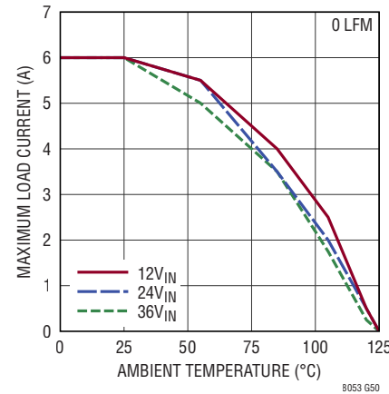
LTM8053 Derating, V_{OUT} = 1.5\text{V} , BIAS = 5V, DC1934A Demo Board
