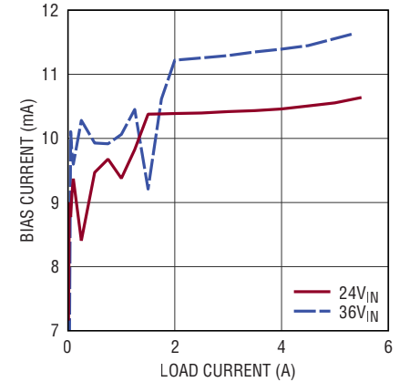
LTM8053 BIAS Current vs Load Current, V_{OUT} = 12V , BIAS = 5V
