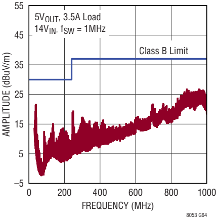
LTM8053 CISPR22 Class B Emissions DC1934A Demo Board, No EMI Filter ( C_{10} = 0.1\mu\text{F} , Short L1, Open C7)
