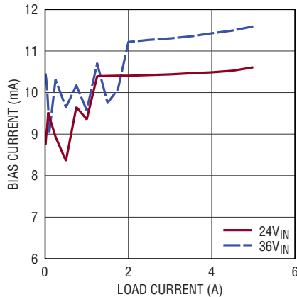
LTM8053 BIAS Current vs Load Current, V_{OUT} = 15V , BIAS = 5V
