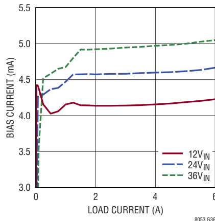
LTM8053 BIAS Current vs Load Current V_{OUT} = 1.8\text{V} , BIAS = 5V
