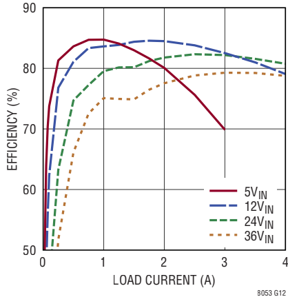
LTM8053 Efficiency vs Load Current, V_{OUT} = -12\text{V} , BIAS Tied to LTM8053 GND
