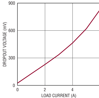
LTM8053 Dropout Voltage vs Load Current, V_{OUT} = 5V , BIAS = 5V
