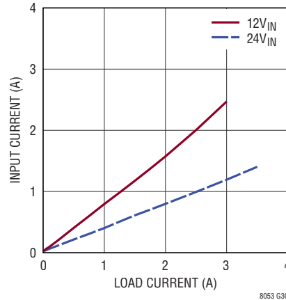
LTM8053 Input vs Load Current V_{OUT} = -8\text{V} , BIAS Tied to LTM8053 GND
