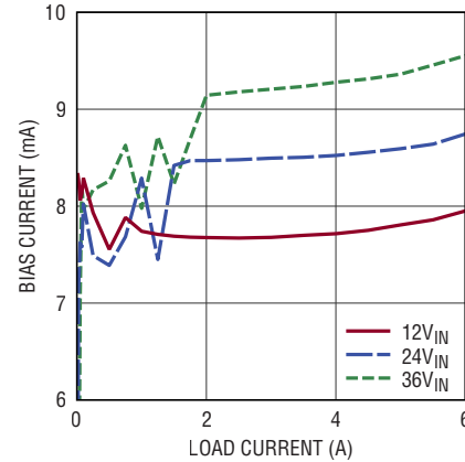
LTM8053 BIAS Current vs Load Current, V_{OUT} = 8V , BIAS = 5V
