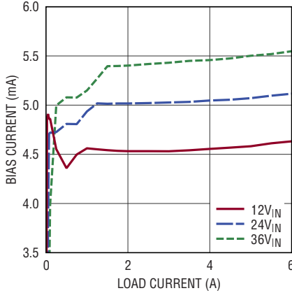
LTM8053 BIAS Current vs Load Current, V_{OUT} = 2V , BIAS = 5V
