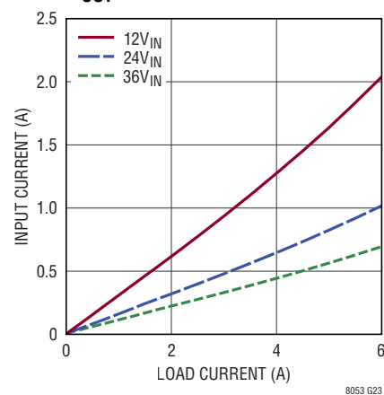
LTM8053 Input vs Load Current V_{OUT} = 3.3\text{V} , \text{BIAS} = 5\text{V}
