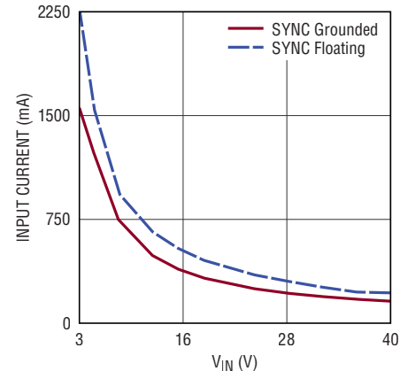
LTM8053 Input Current vs V_{IN} , V_{OUT} Short-Circuited
