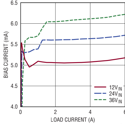
LTM8053 BIAS Current vs Load Current, V_{OUT} = 2.5V , BIAS = 5V
