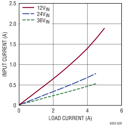
LTM8053 Input vs Load Current V_{OUT} = -12\text{V} , BIAS tied to LTM8053 GND
