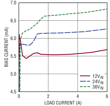
LTM8053 BIAS Current vs Load Current, V_{OUT} = 3.3V , BIAS = 5V
