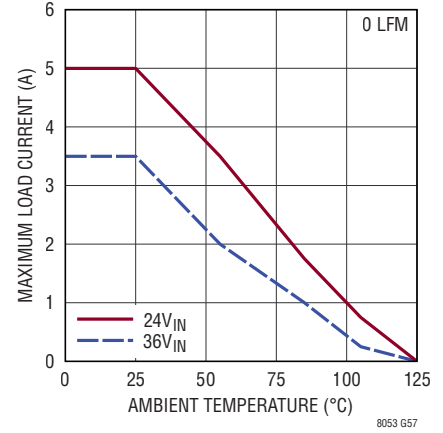
LTM8053 Derating, V_{OUT} = -3.3\text{V} , BIAS Tied to LTM8053 GND, DC1934A Demo Board
