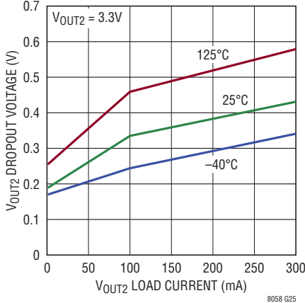
V_{OUT2} Dropout
