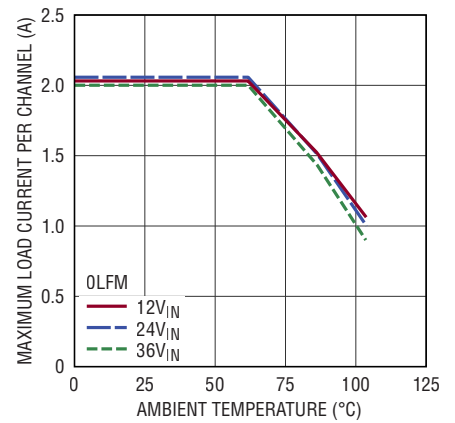
Derating, V_{OUT} = 1.8\text{V} , \text{BIAS} = 5\text{V} , DC2777A Demo Board Both Channels at Same Load
