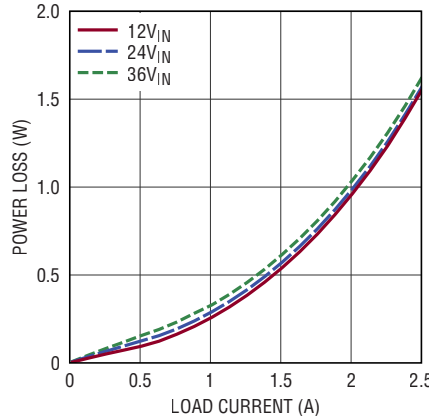
Power Loss, V_{OUT} = 0.8V BIAS = 5V, Burst Mode Operation
