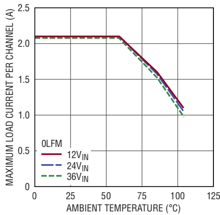
Derating, V_{OUT} = 0.8\text{V} \text{BIAS} = 5\text{V} , DC2777A Demo Board Both Channels at Same Load
