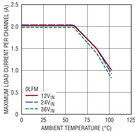
Derating, V_{OUT} = 1.5\text{V} \text{BIAS} = 5\text{V} , DC2777A Demo Board Both Channels at Same Load
