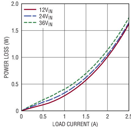
Power Loss, V_{OUT} = 1.5V BIAS = 5V, Burst Mode Operation
