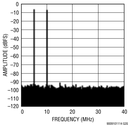
LTM9009-14: 8k Point 2-Tone FFT, f_{IN} = 70\text{MHz} , 75\text{MHz} , -7\text{dBFS} per Tone, 80\text{Mpsps}
