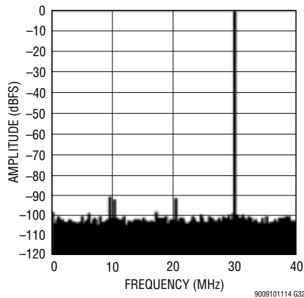
LTM9009-14: 8k Point FFT, f_{IN} = 30\text{MHz} , -1\text{dBFS} , 80\text{Mpsps}
