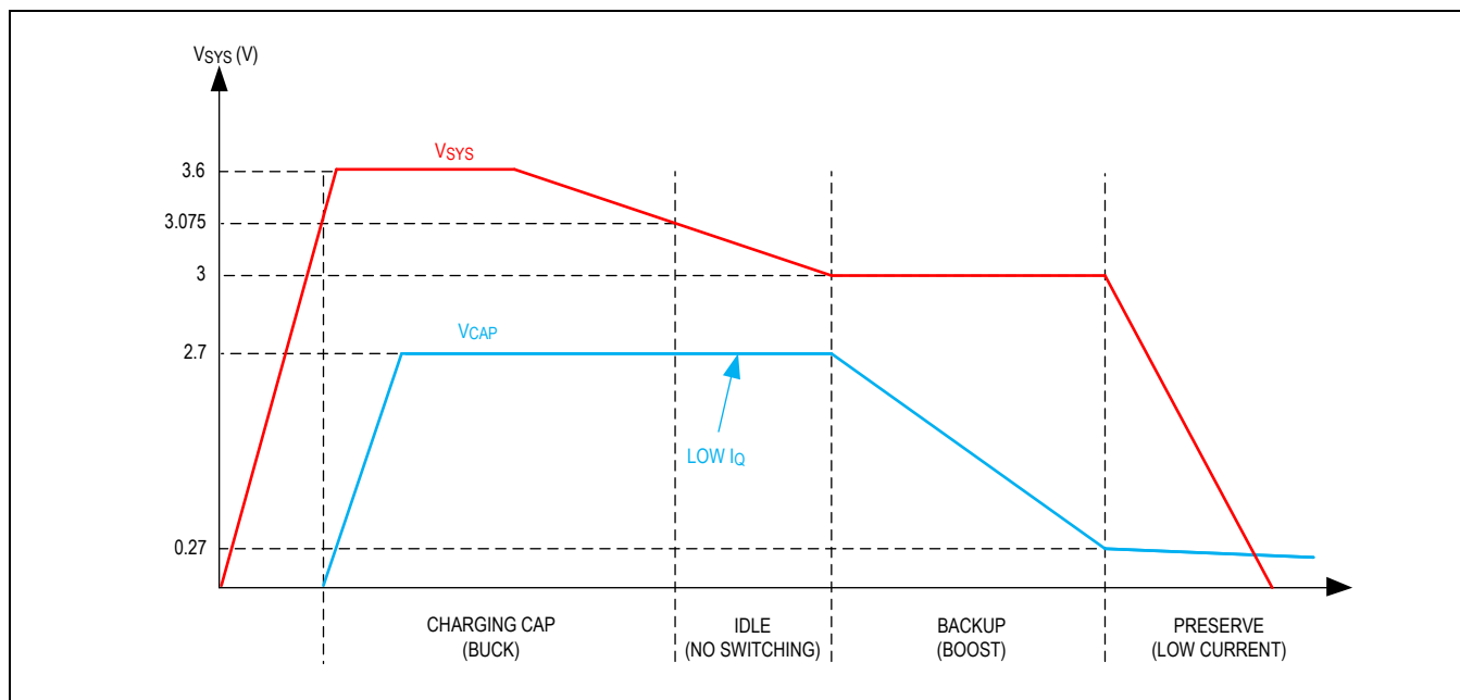
Figure 3. Charging/Discharging Waveforms
