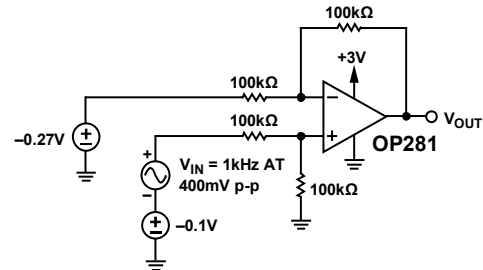
Figure 37. Single OPx81 Channel Configured as a Difference Amplifier Operating at V CM < 0 V
