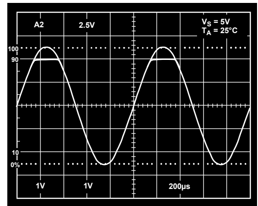
Figure 32. No Phase Reversal
