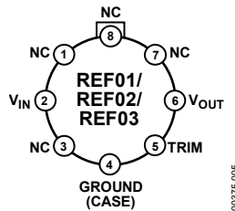
Figure 5. 8-Lead TO-99 (J-Suffix) Pin Configuration
