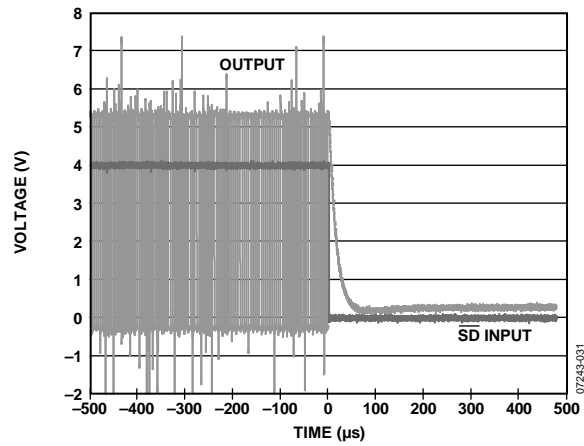
Figure 31. Turn-Off Response
