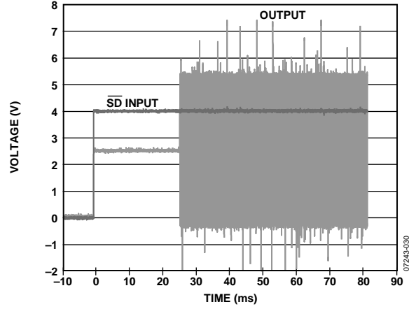
Figure 30. Turn-On Response
