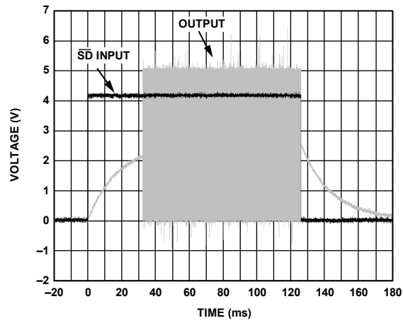
Figure 31. Turn-Off Response
