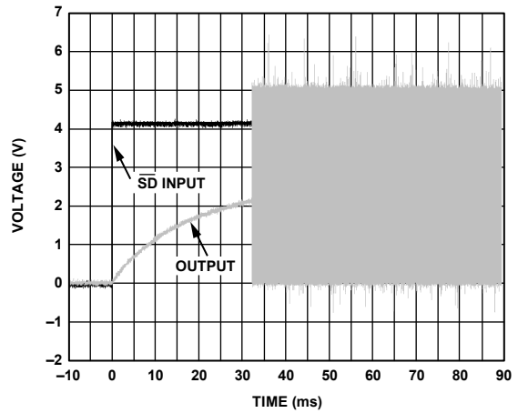
Figure 30. Turn-On Response
