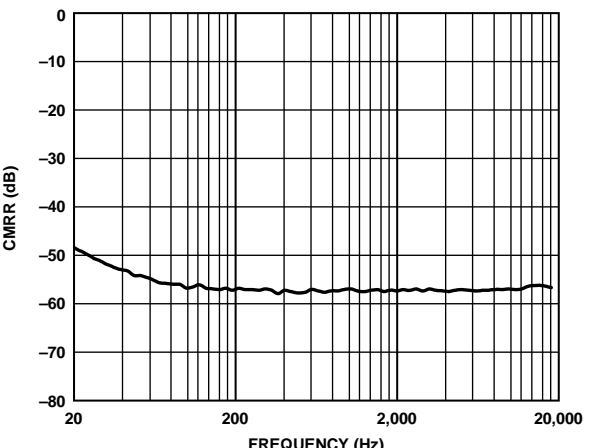
Figure 32. CMRR vs. Frequency, V ripple = 100 mV rms, AC-Coupled
