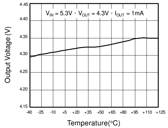
Output Voltage
