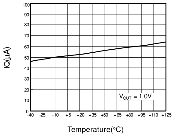
Quiescent Current
