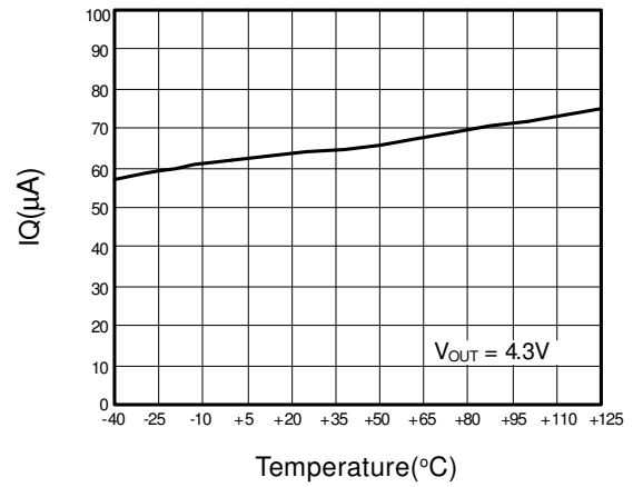
Quiescent Current
