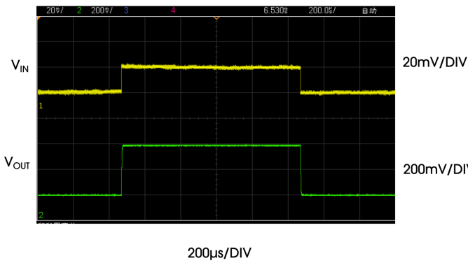
Figure 10. Small Signal Step Response
