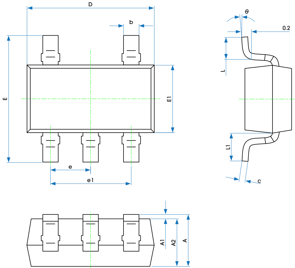
Figure 23. Package View
