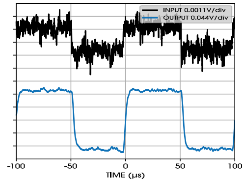
Figure 13. Small Signal Step Response (Gain = 100)
