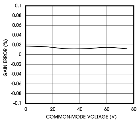
Figure 7. Gain Error vs. Common Mode Voltage
