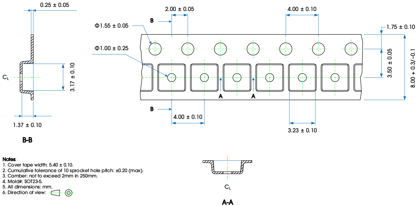
Figure 24. Carrier Tape Drawing
