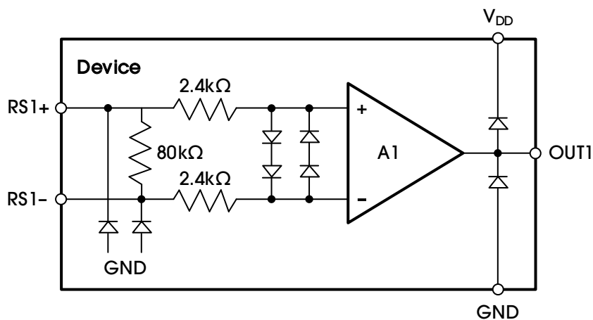
Figure 22. Functional Block Diagram
