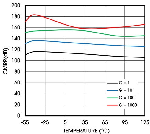
Figure 12. CMRR vs. Temperature
