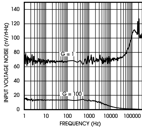
Figure 17. Input Voltage Noise Density
