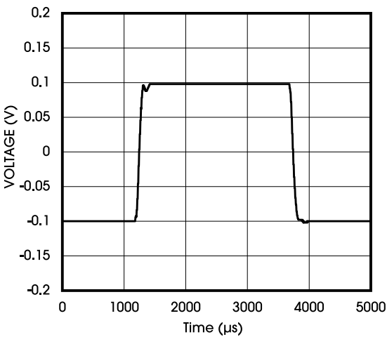
Figure 24. Small Signal Pulse Response, 5V
