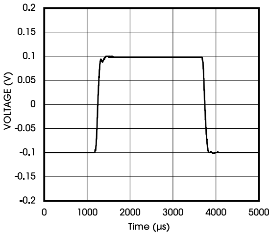
Figure 20. Small Signal Pulse Response, 1.8V
