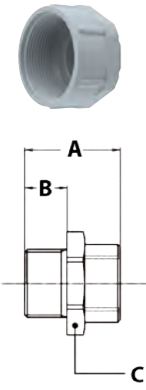
Pg / Pg enlarger, glassfiber reinforced polyamide, colour grey
