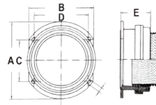
GIGANT straight flange fitting, colour grey, male, PA6, IP 54 (with 4 fixing holes Ø 6,5 mm)
