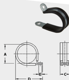
Conduit mounting clip, galvanised steel
