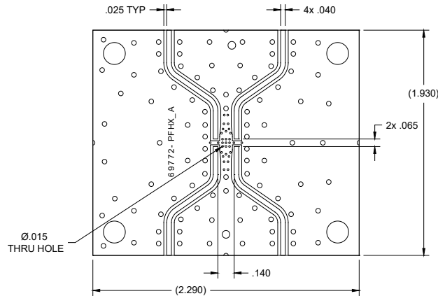
2dB- 5dB Coupler Test Board
