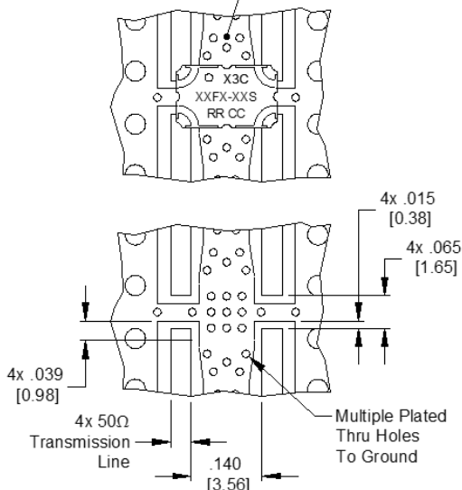
Dimensions are in Inches [Millimeters] X3CXXFX-XXS Mounting Footprint
