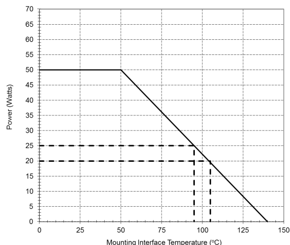
X3C14F1-03 Power Derating Curve
