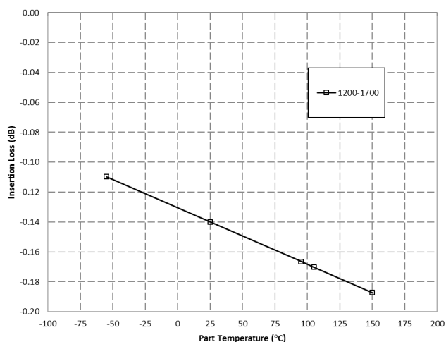
X3C14F1-03S Typical Insertion Loss Derating Curve
