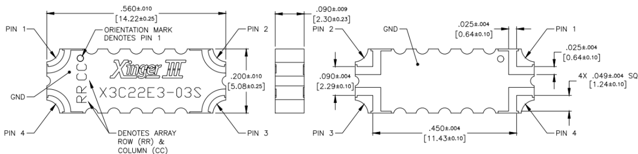
Dimensions Are in Inches [Millimeters] X3C22E3-03S Mechanical Outline
