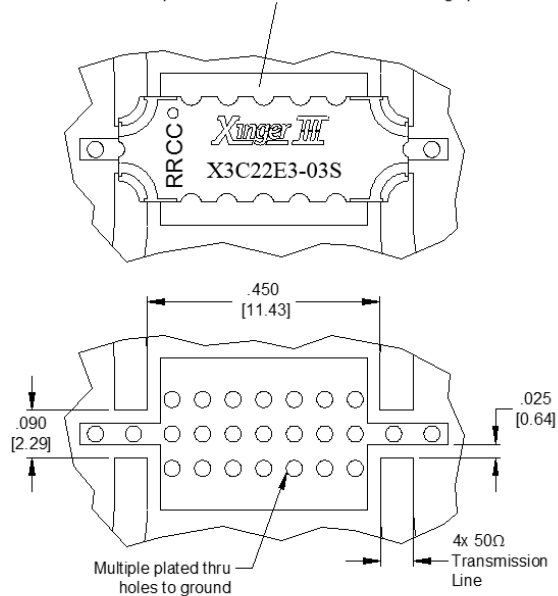
Dimensions Are in Inches [Millimeters] X3C22E3-03S Mounting Footprint
