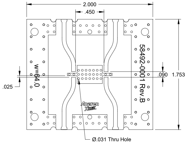
3 dB and 5dB Test Board
