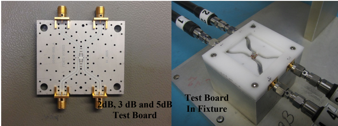
Test Station
