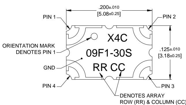
Dimensions are in Inches [Millimeters] X4C09F1-30S Mechanical Outline
