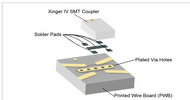
Figure 5: Mounting Features Example
