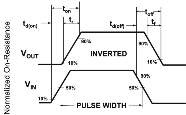
Figure 2: Switching Waveforms
