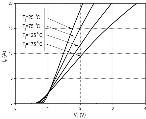
Figure 1. Forward Characteristics
