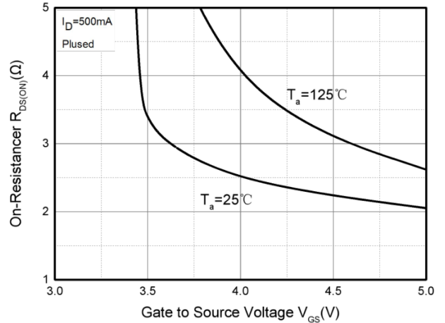
RDS(ON)—VGS
