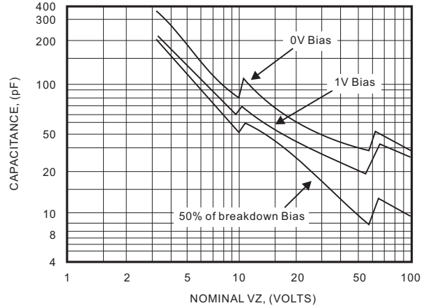
Fig 5. Capacitance Curve
