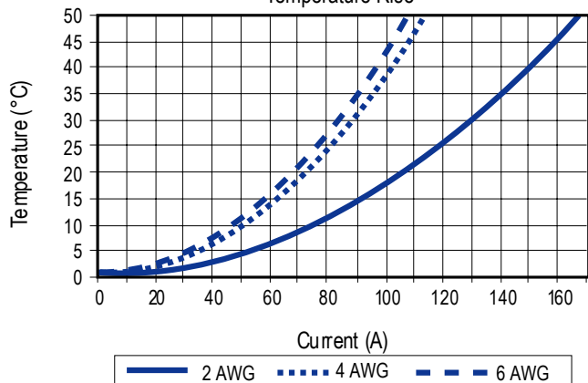
PowerMod®HP Dual Pole Series "A" Temperature Rise
