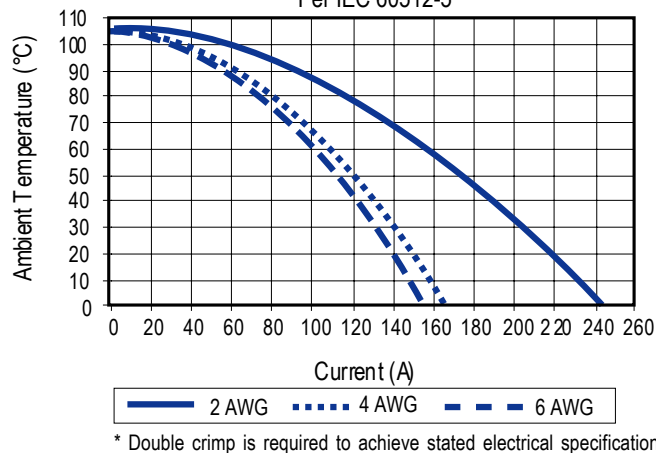
PowerMod®HP Dual Pole De-rating Curve Series "A" Per IEC 60512-5
