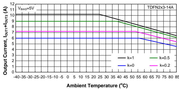
Figure 3. Derating Curves for APL3523 Package
