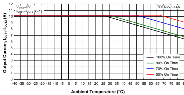
Figure 4. Safe Operating Area for APL3523 Package
