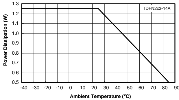
Figure 3. Derating Curves for APL3523 Package
