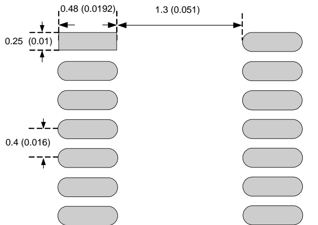
TDFN2x3-14A
